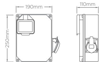
RE113F Enclosure
