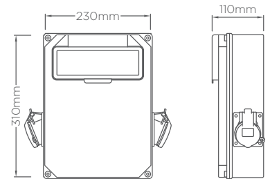
RE115F Enclosure
