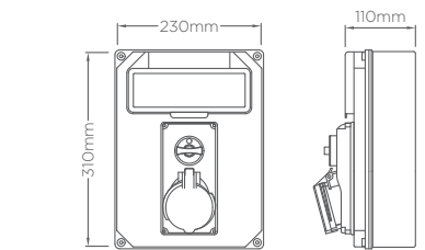
RE115F Enclosure
